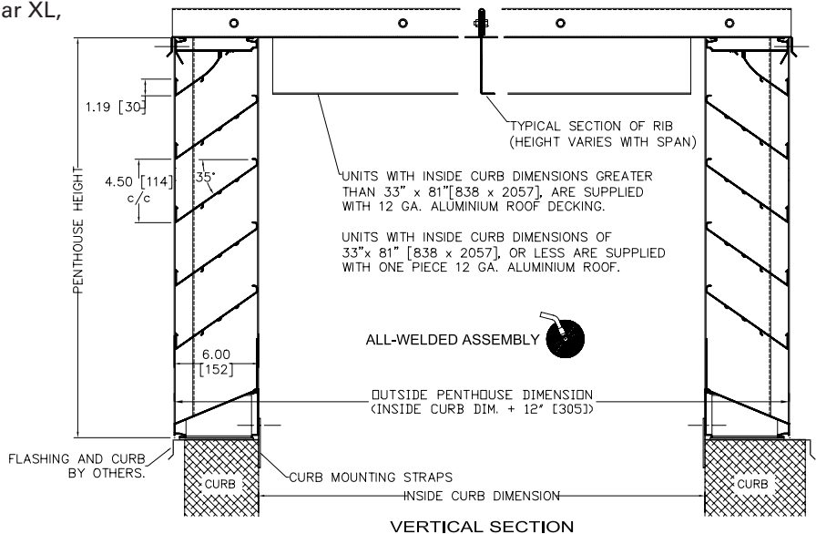
VERTICAL SECTION
